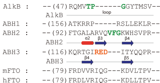
FIGURE 8. Structure–sequence alignment of the AlkB-family proteins in the region containing the base-flipping hairpin motif in ABH2 and ABH3.
